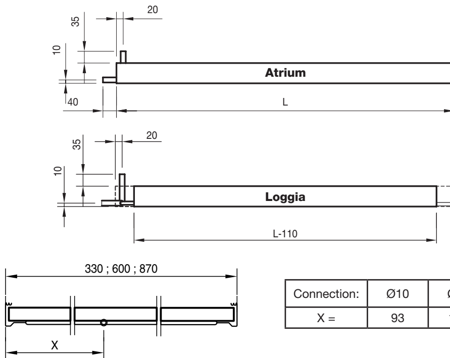
Figure 4.b. Atrium and Loggia dimensions, water connection and connection.
