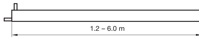
Figure 4. Atrium and Loggia are manufactured as standard in lengths from 1.2 m to 6.0 m in steps of 0.1 m. Actual length dimension is -12 mm.
