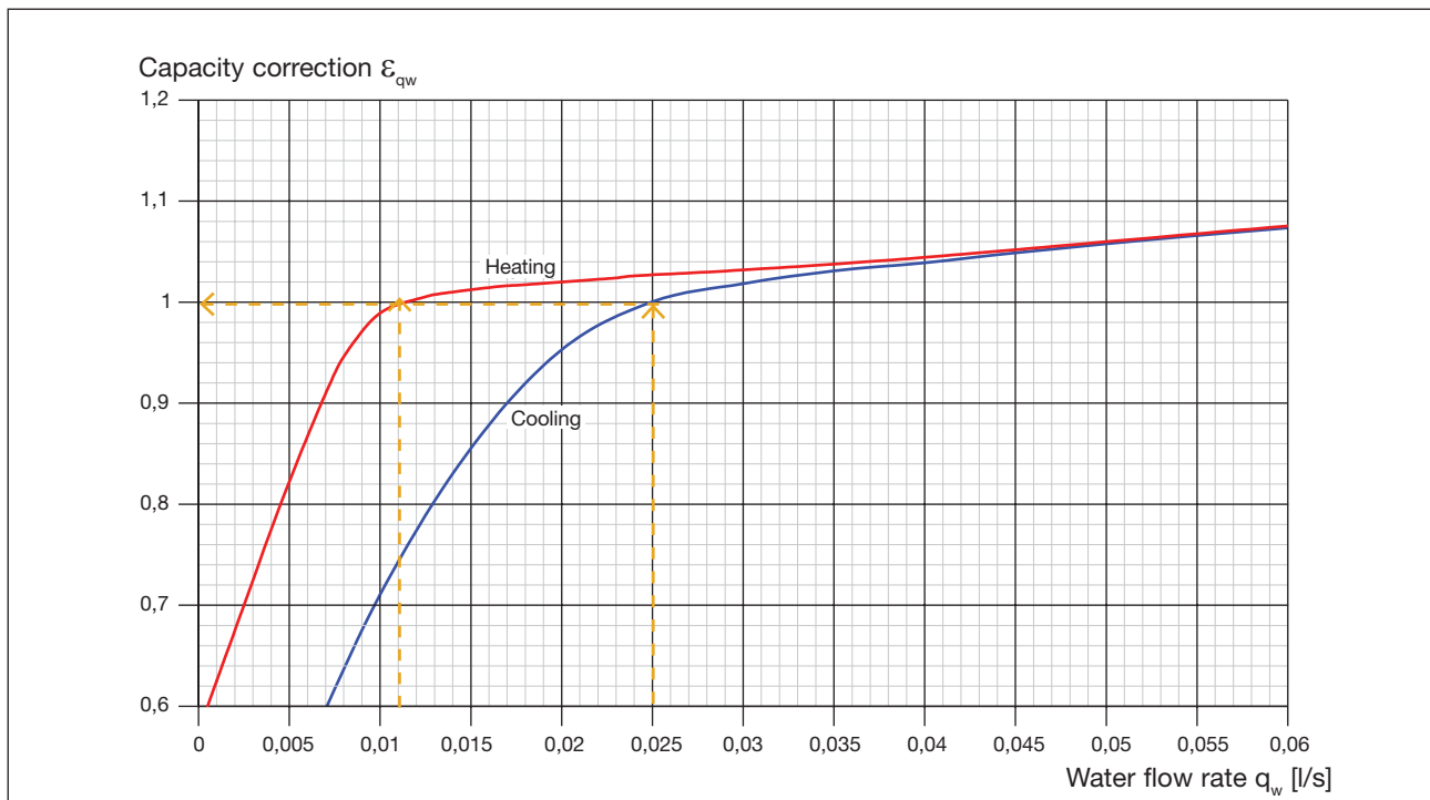
Diagram 3. Capacity correction \varepsilon_{q_w} as a function of water flow rate q_w .
