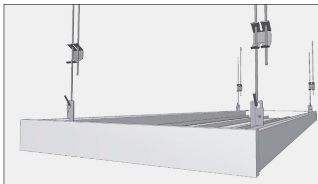
Figure 8. Atrium suspended with adjustable pendulum hangers in combination with Atrium panel hooks.
