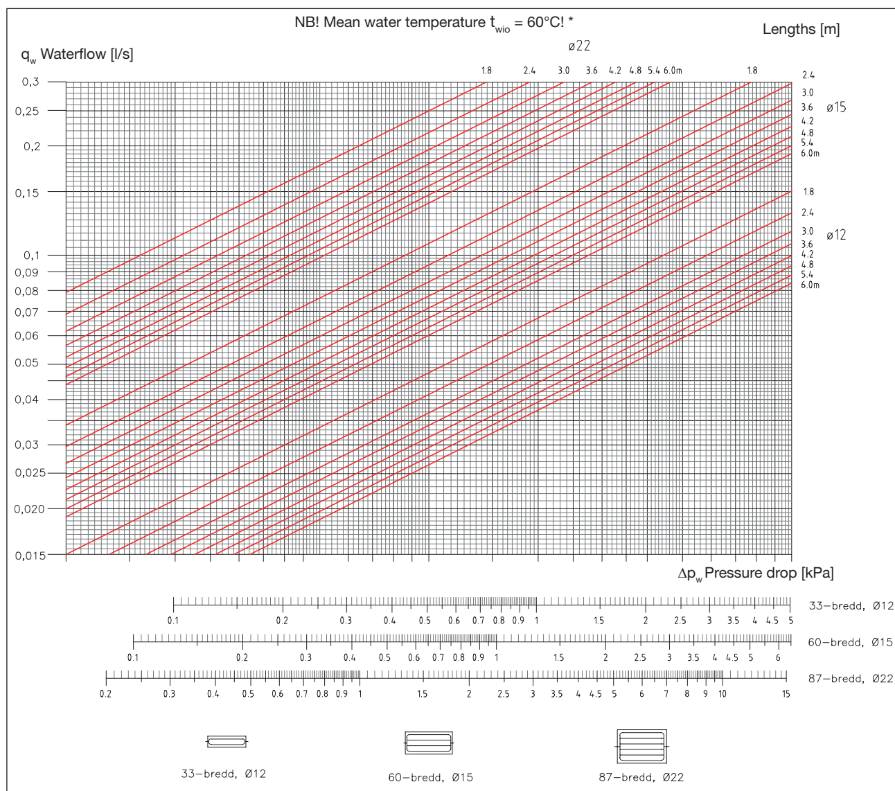
Diagram 5. Panels, pressure drop at 60°C. For pressure drops at temperatures other than 60°C, the pressure drop is multiplied by the pressure drop factor (see diagram 7).
